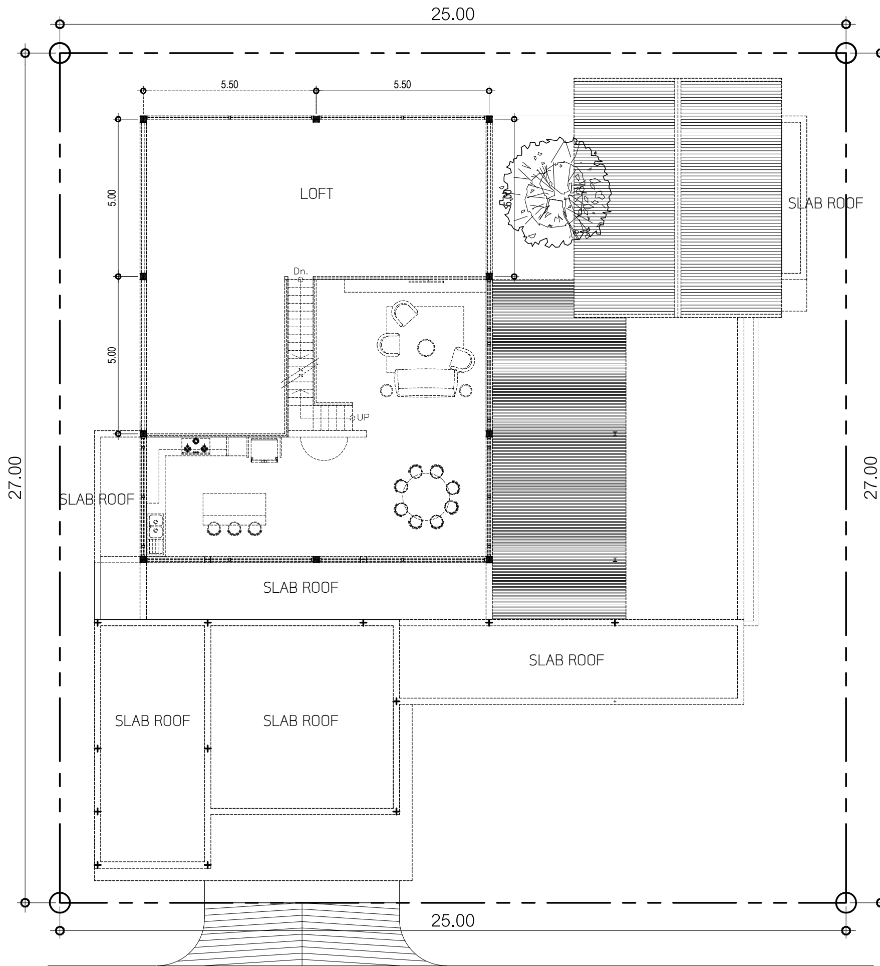
LOFT FLOOR PLAN
